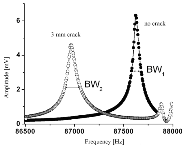
Figure 3.1 Si wafer/cell with crack (open marks) can be separated from a regular wafer/cell (closed marks) using one of three rejection criteria: (1) reduced amplitude, (2) increased bandwidth (BW), and (3) resonance downward frequency shift [31].
