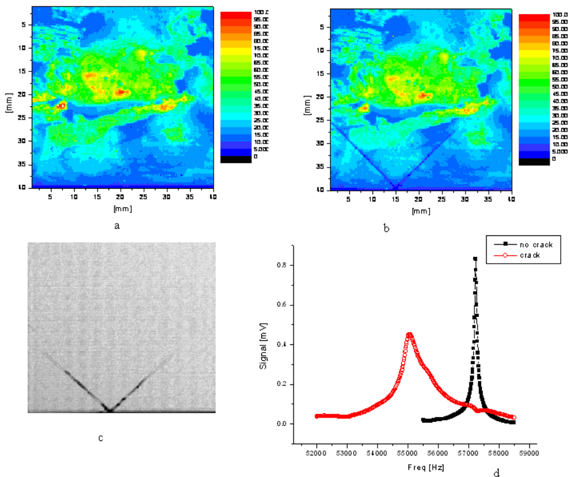
Figure 3.13 a – PL map of area before crack 40 x 40 mm at room temperature and 1126 nm wavelength, intensity shown from 0 mV – blue to 100 mV – red; b – PL map with crack 17.7 x 24.5 mm of the same area; c – SAM image 40 x 40 mm, resolution 10 microns; d – RUV parameters shift on the same wafer before the crack (closed marks) and after the crack (opened marks).
